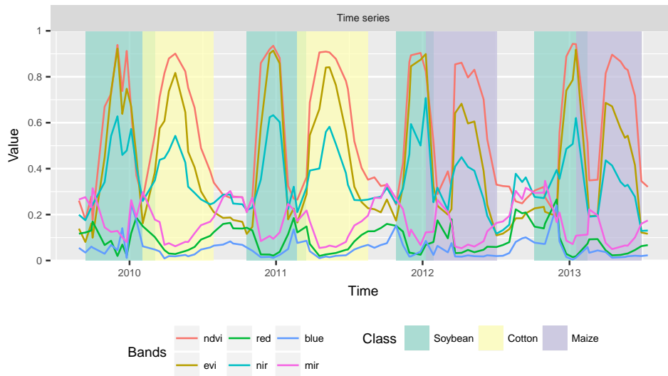
Figure 8: Classification of each 6 months periods of the time series using results of the TWDTW analysis with logistic time-weight. The solid lines are the attributes of the time series, the background colors indicate the classification of the periods.
