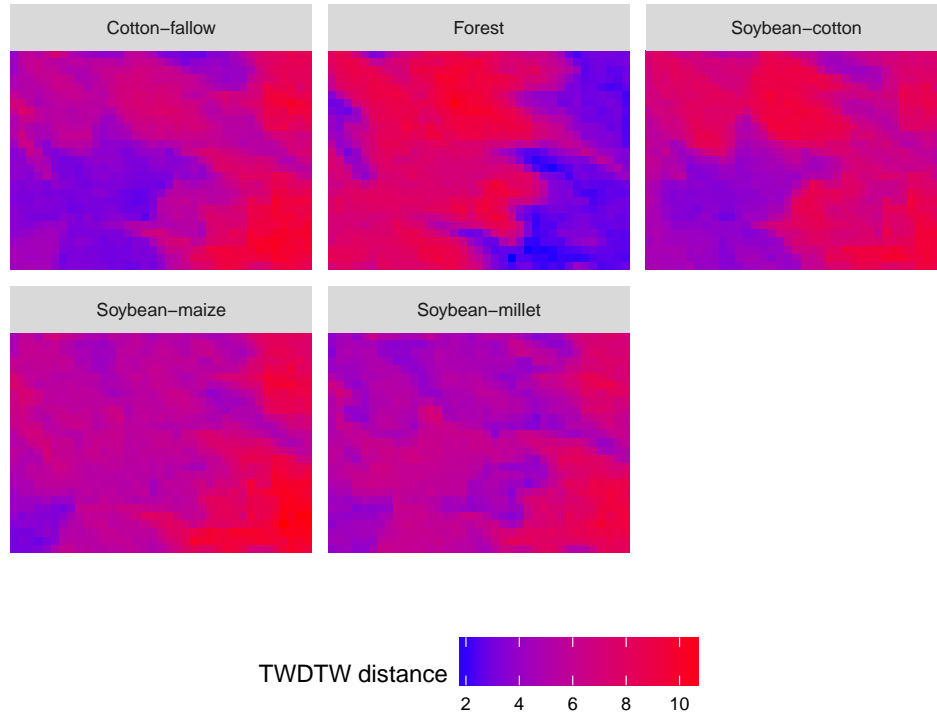
Figure 12: Illustration of the TWDTW dissimilarity from each temporal pattern in 2008. The blue areas are more similar to the pattern and the red areas are less similar to the pattern.
